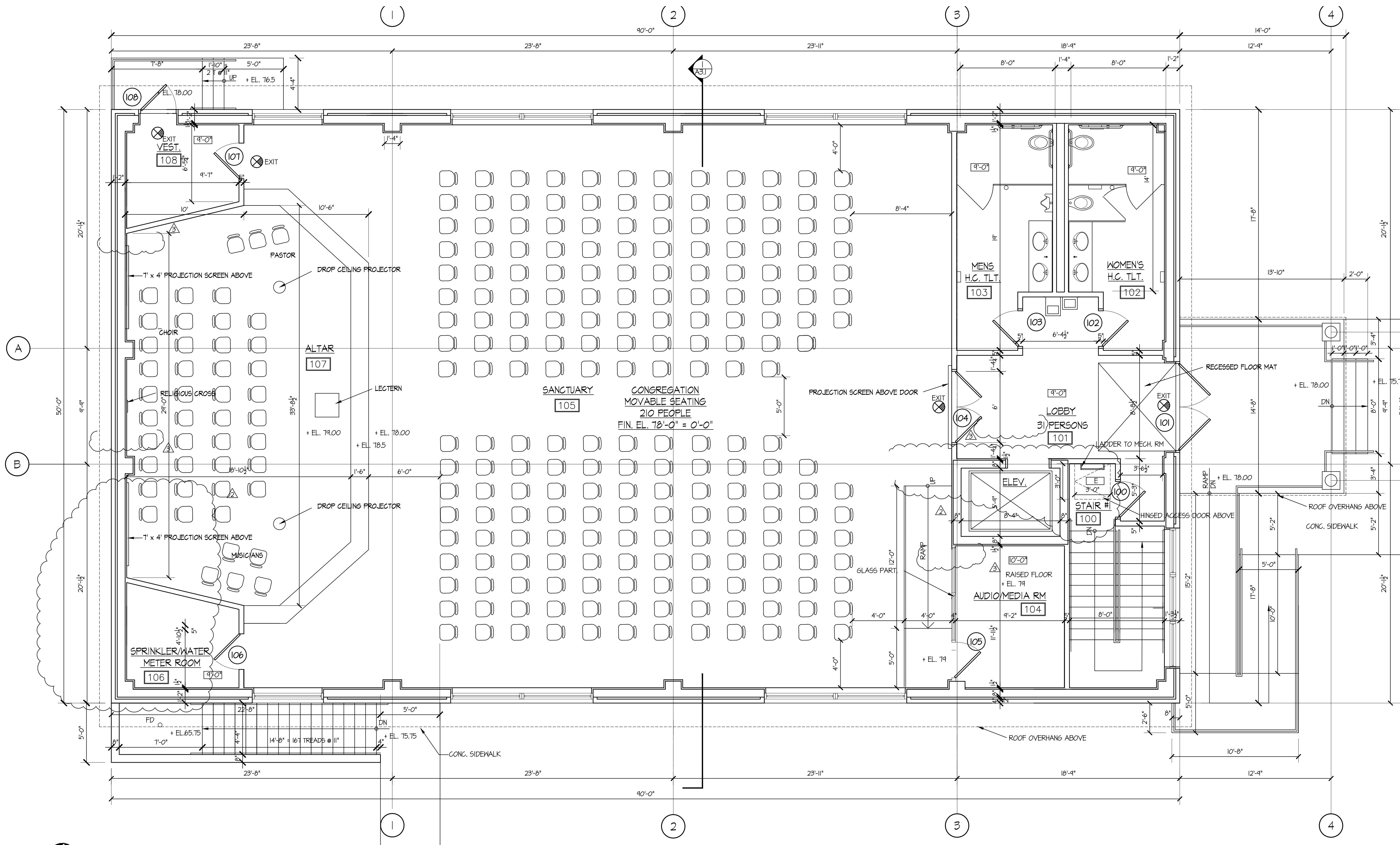
PROPOSED FIRST FLOOR PLAN SCALE: 1/4" = 1'-0"
